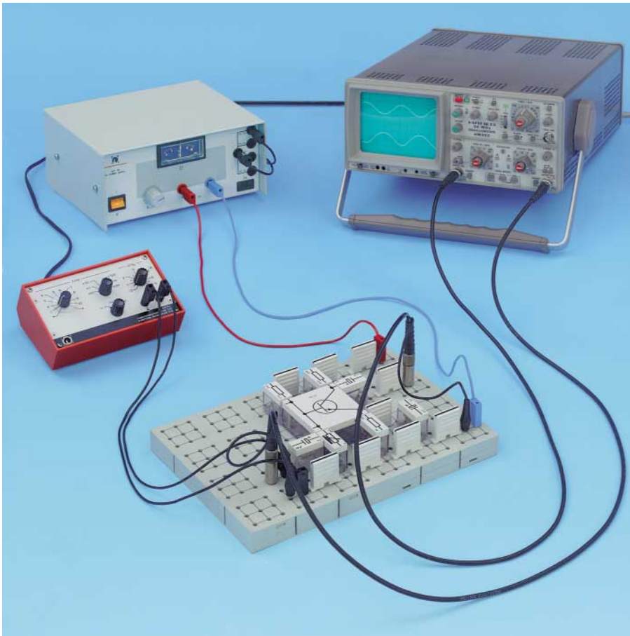
Transistor as amplifier (P 4.1.6.1)
